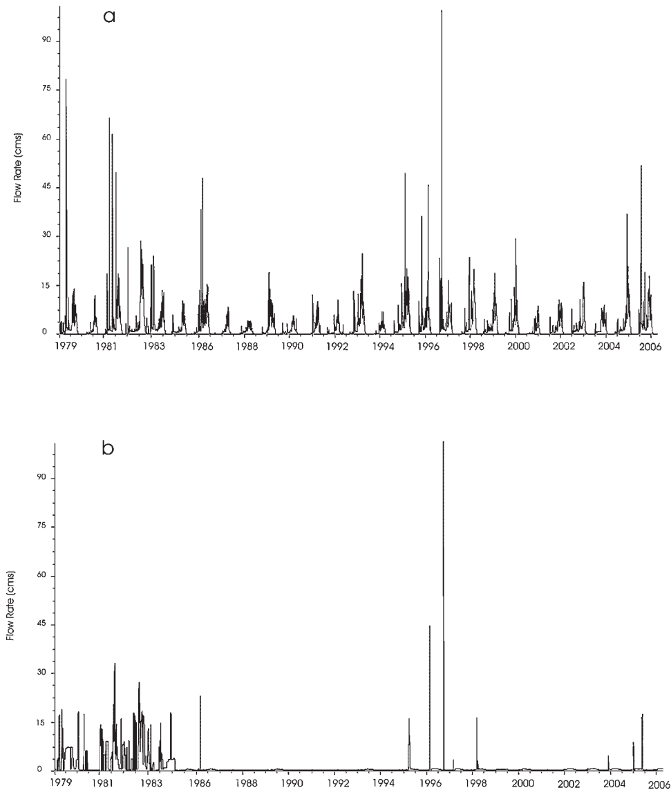
Figure 4. Example 25-year hydrographs of west slope Sierra Nevada streams in this study: (a) Cole Creek, an unregulated stream with normal seasonal fluctuations; (b) South Fork Silver Creek below Ice House Reservoir, a regulated stream with reduced seasonal fluctuations
