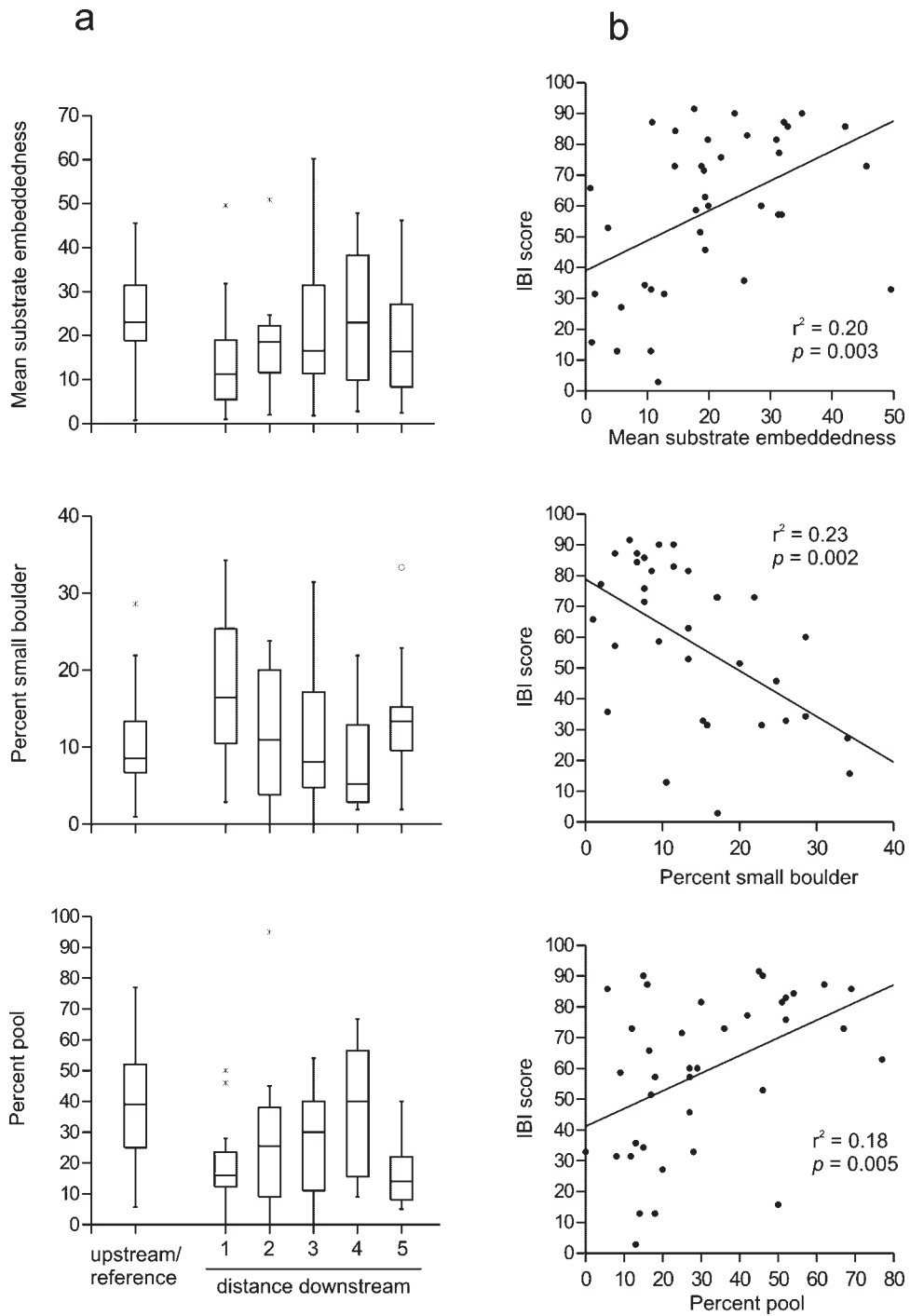
Figure 3. (a) Box-and-whisker plots of the few PHAB variables that showed similar response with proximity to dam as did final BMI metrics and the IBI. Per cent sand was redundant with mean substrate embeddedness but showed the same response. Boxes indicate median values and interquartile ranges, whiskers indicate 95th percentiles, outliers are indicated by an x; (b) scatterplots and least squares regressions of IBI on the same PHAB variables as in (a) based on reference and first downstream sites only
